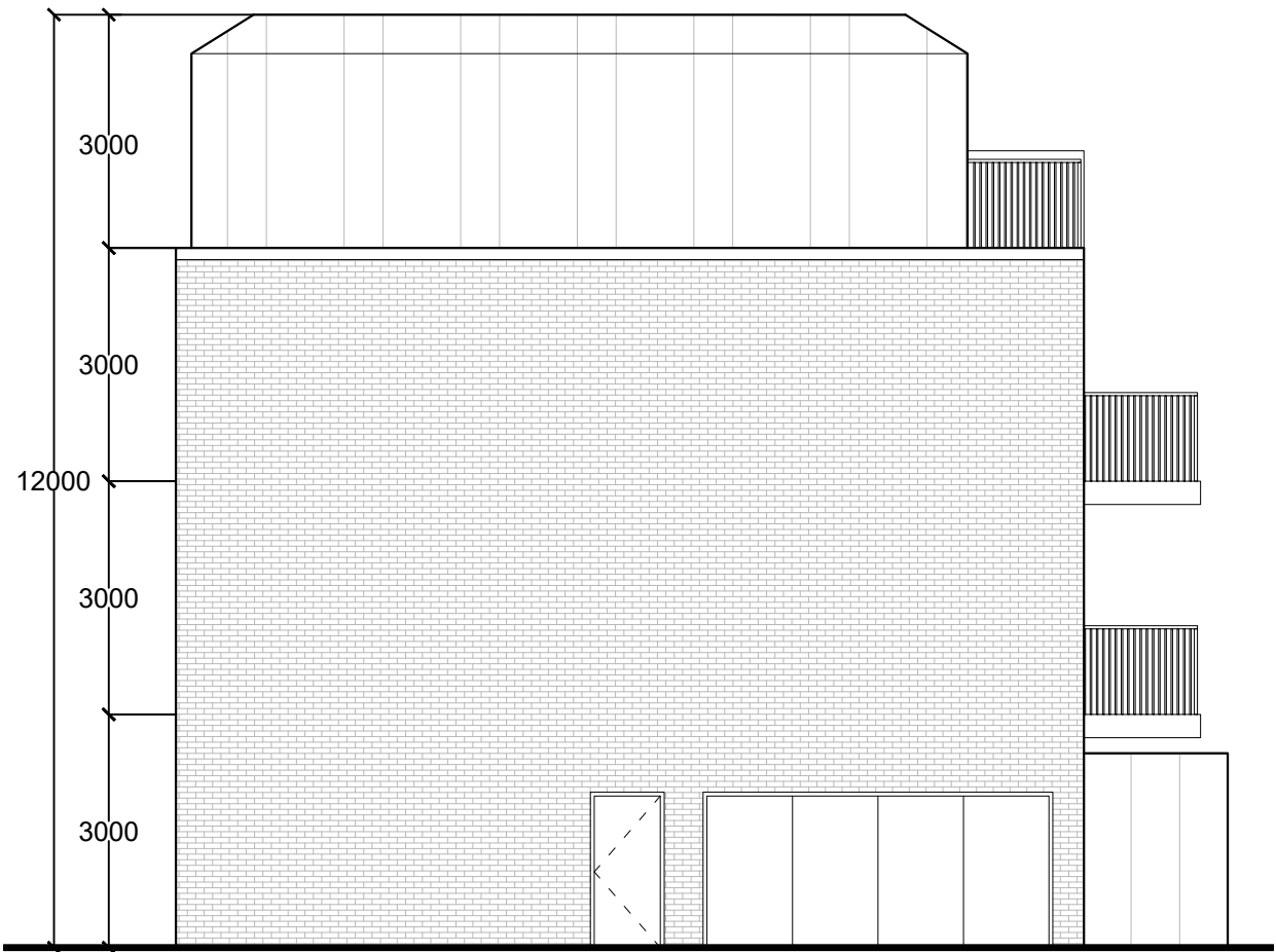
Side (East) Elevation
