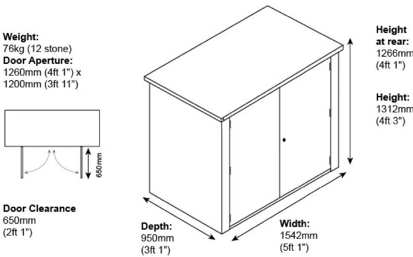
VANGUARD GARDEN SHED EXTERNAL MEASUREMENTS
