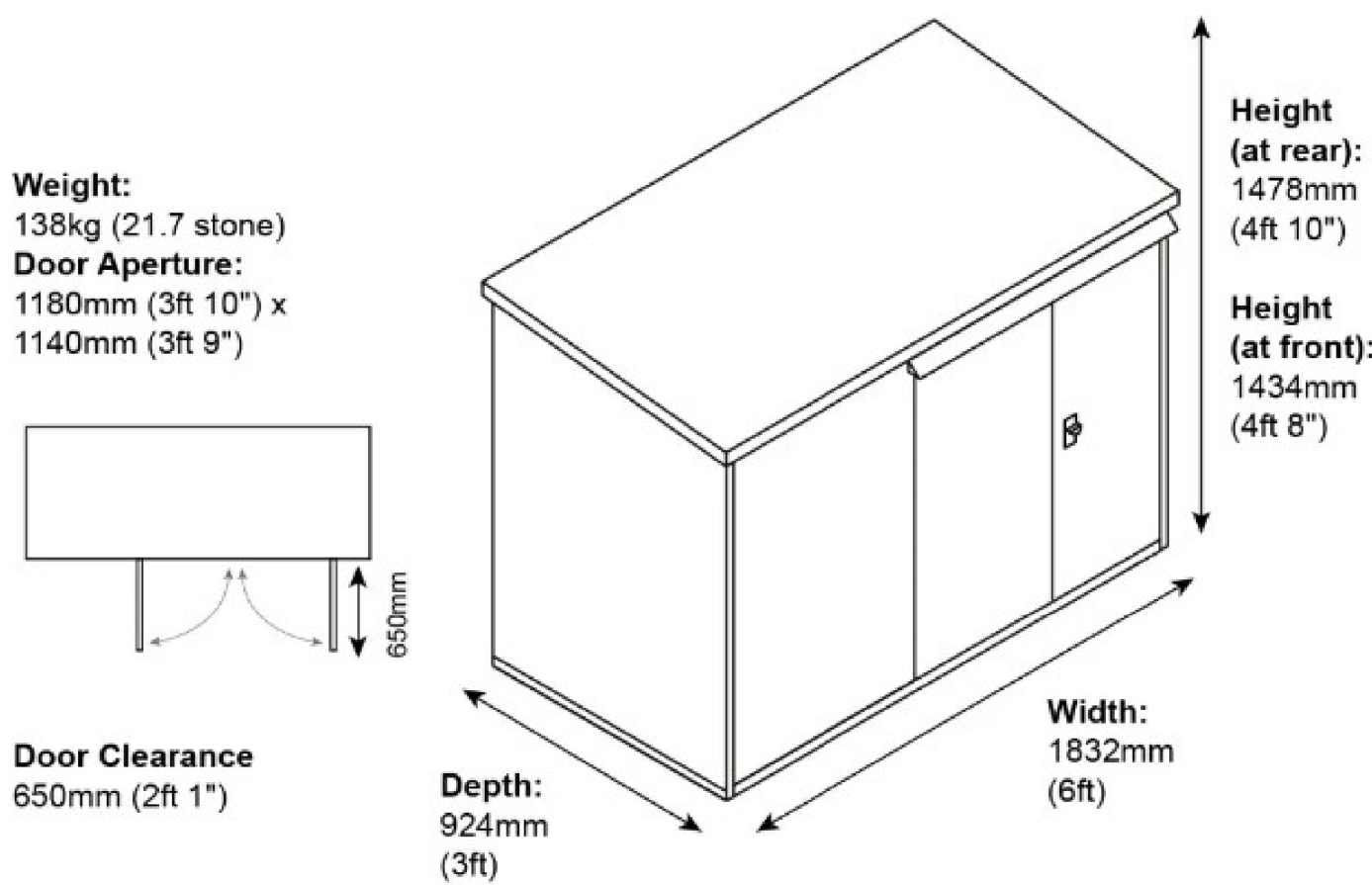
ANNEXE (HIGH SECURITY) BIKE SHED x3 EXTERNAL MEASUREMENTS
