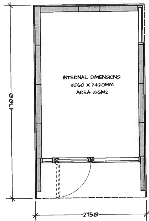
PLAN EXTERNAL DIMENSIONS: 4700 X 2750MM AREA: 12.9M 2
