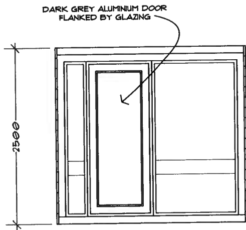
A-A: CABIN WEST ELEVATION
