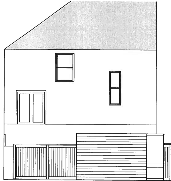
(E2) SOUTH ELEVATION PROPOSAL
