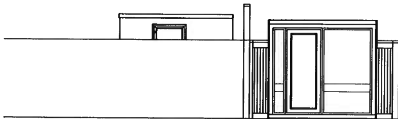
(E3) WEST ELEVATION PROPOSAL
