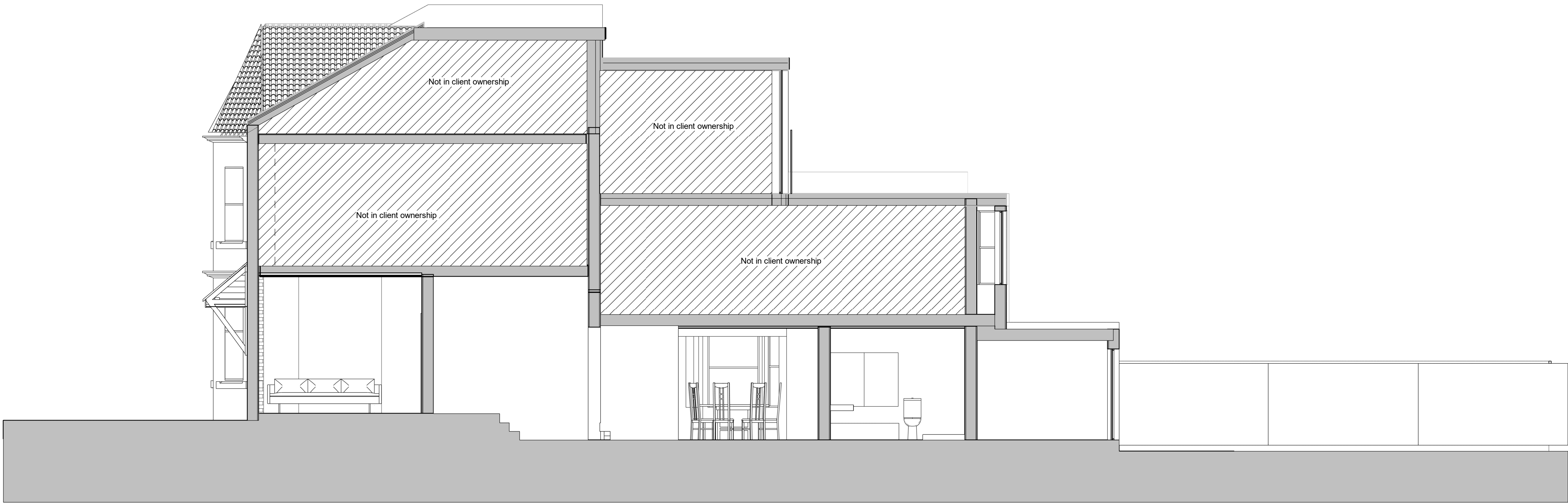
Existing Building Section 1 : 50
