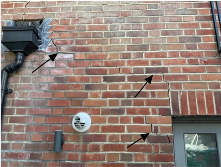
Cracking to front elevation
