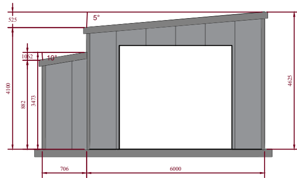
Front Elevation (External)
