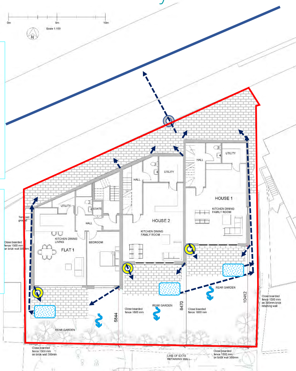
Figure 1. Proposed SuDS scheme layout
