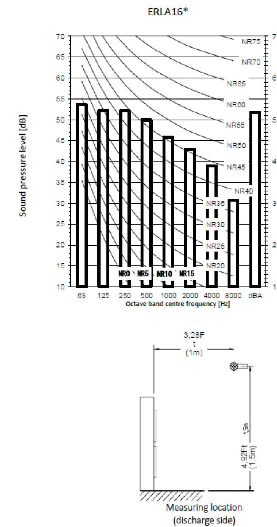
04 SOUND PRESSURE LEVEL - HEAT PUMP CONDENSER
