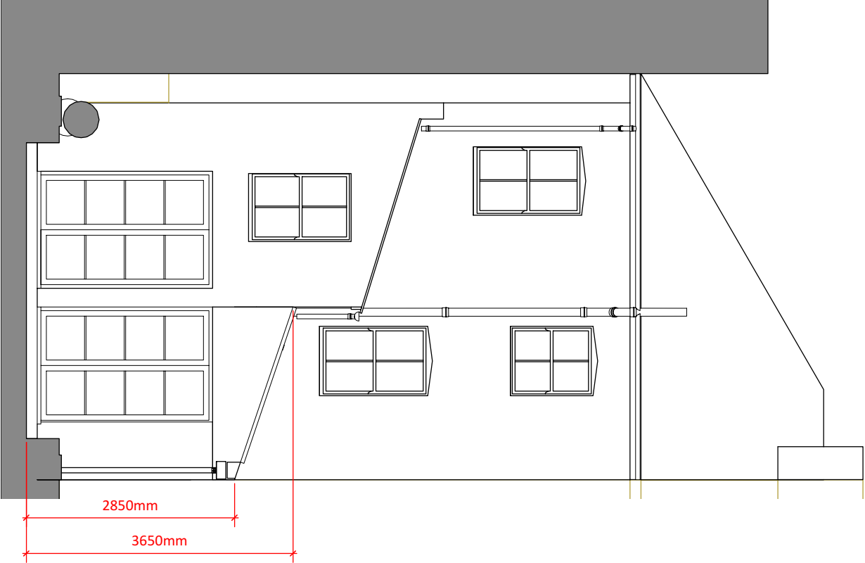
Rear Elevation - Proposed 1:50
