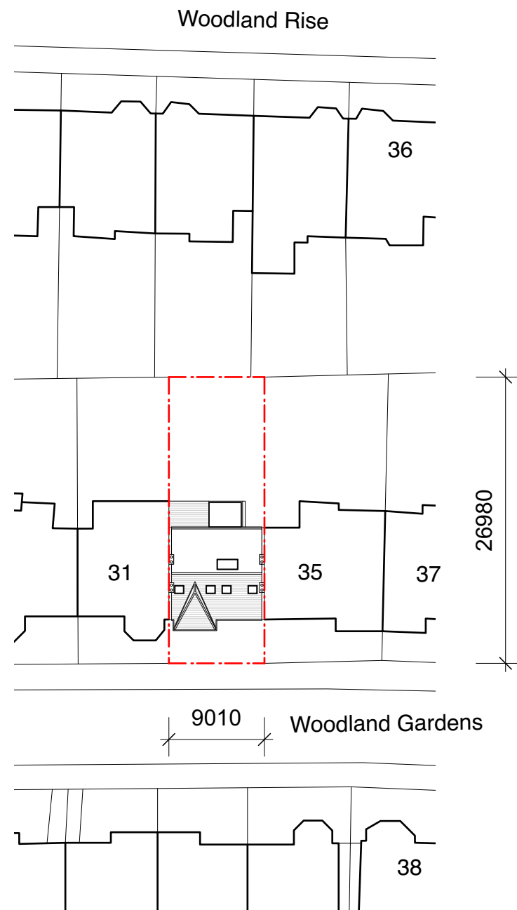
Approved Block Plan
