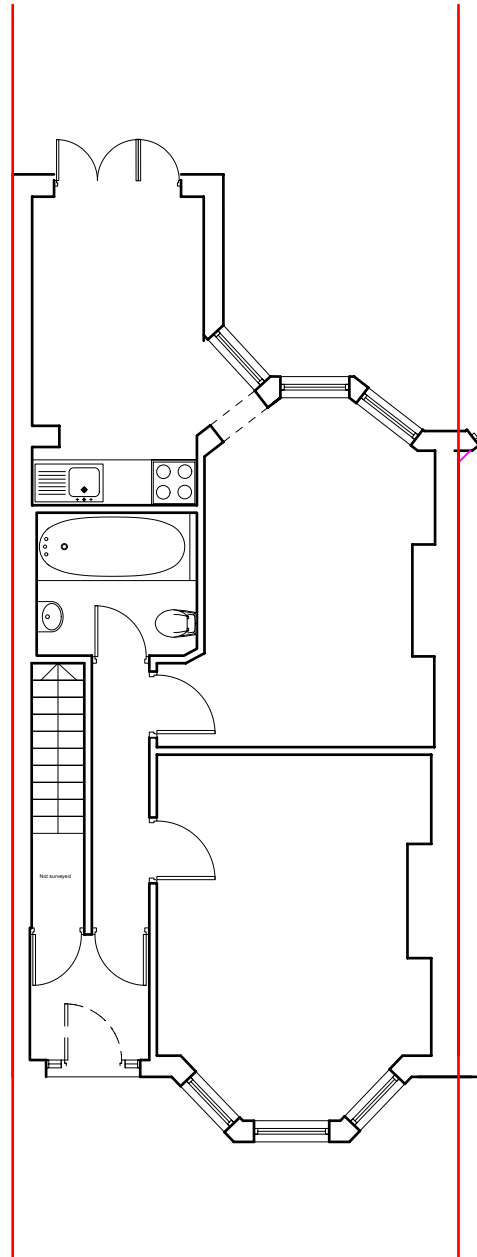
Ground floor Existing plan
