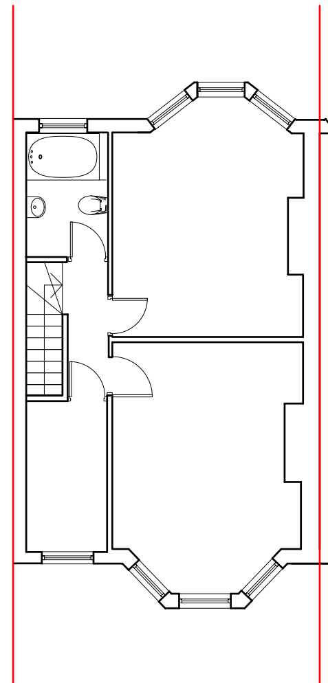
First floor Proposed plan
