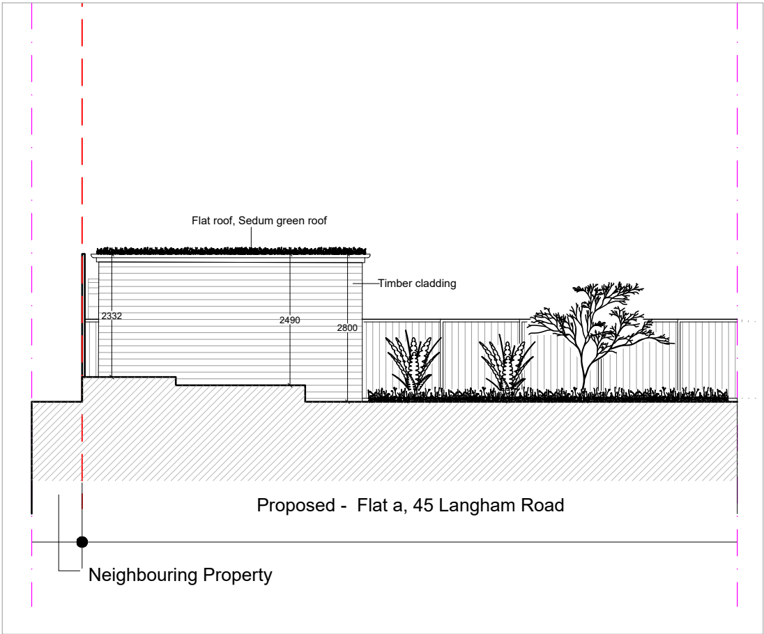
Side Elevation 1
