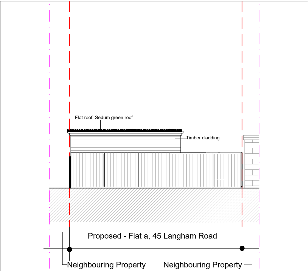
Rear Elevation
