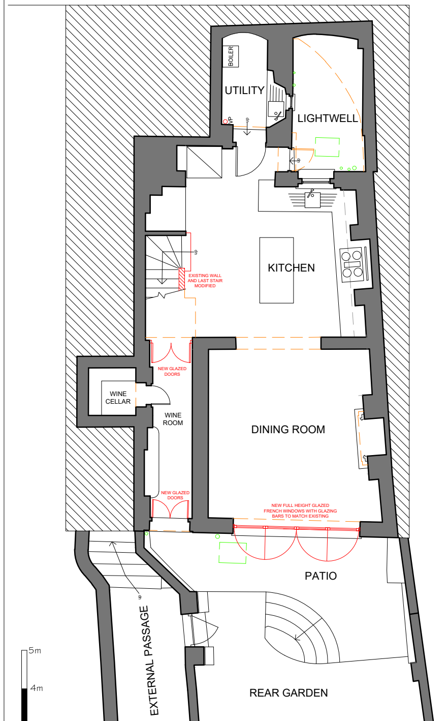
LOWER GROUND FLOOR PLAN
