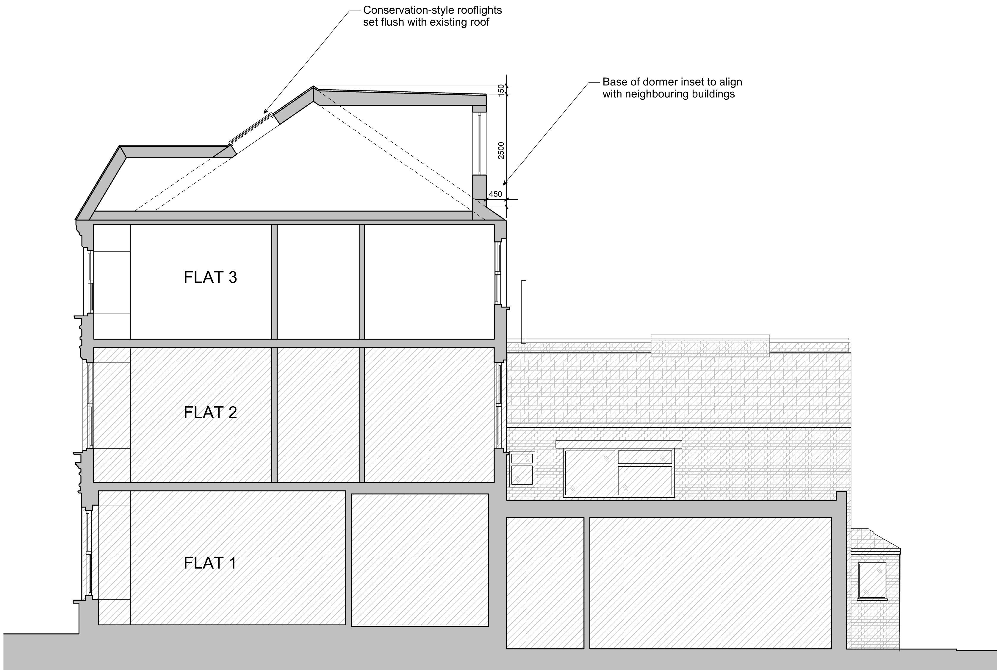
01 Section - Proposed
