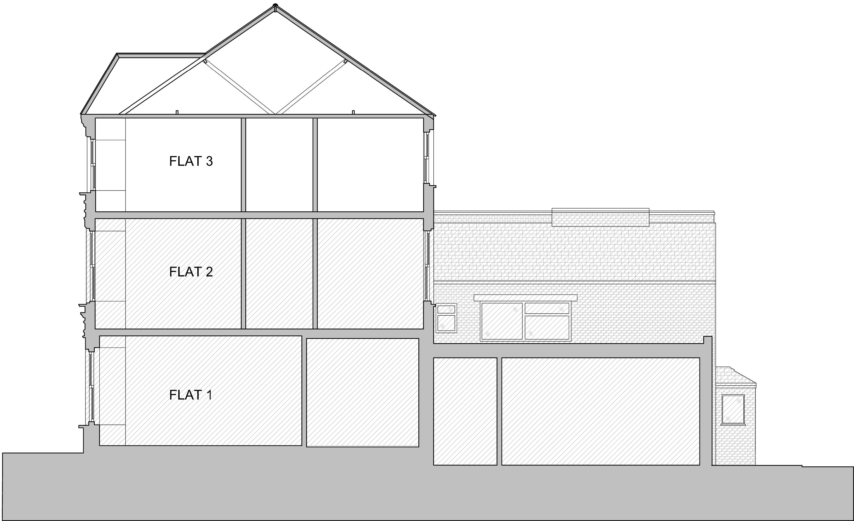
01 Section - Existing
