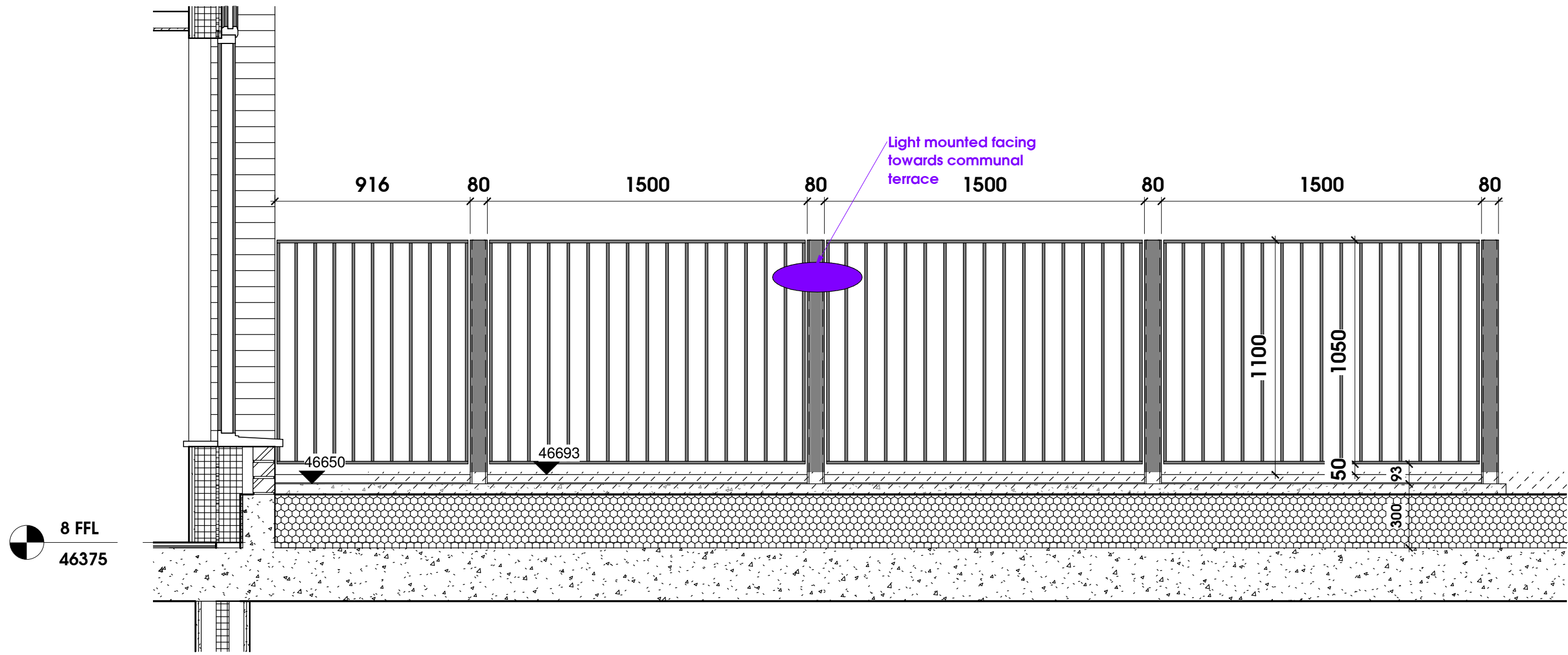
2 8th Floor Railing Elevation 3 1 : 20
