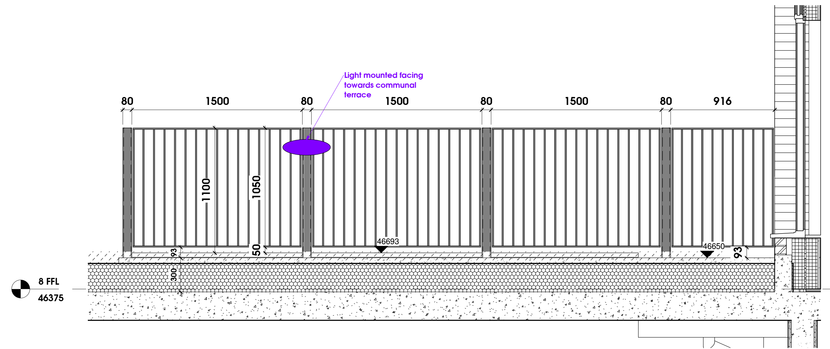
1 8th Floor Railing Elevation 1 1 : 20
