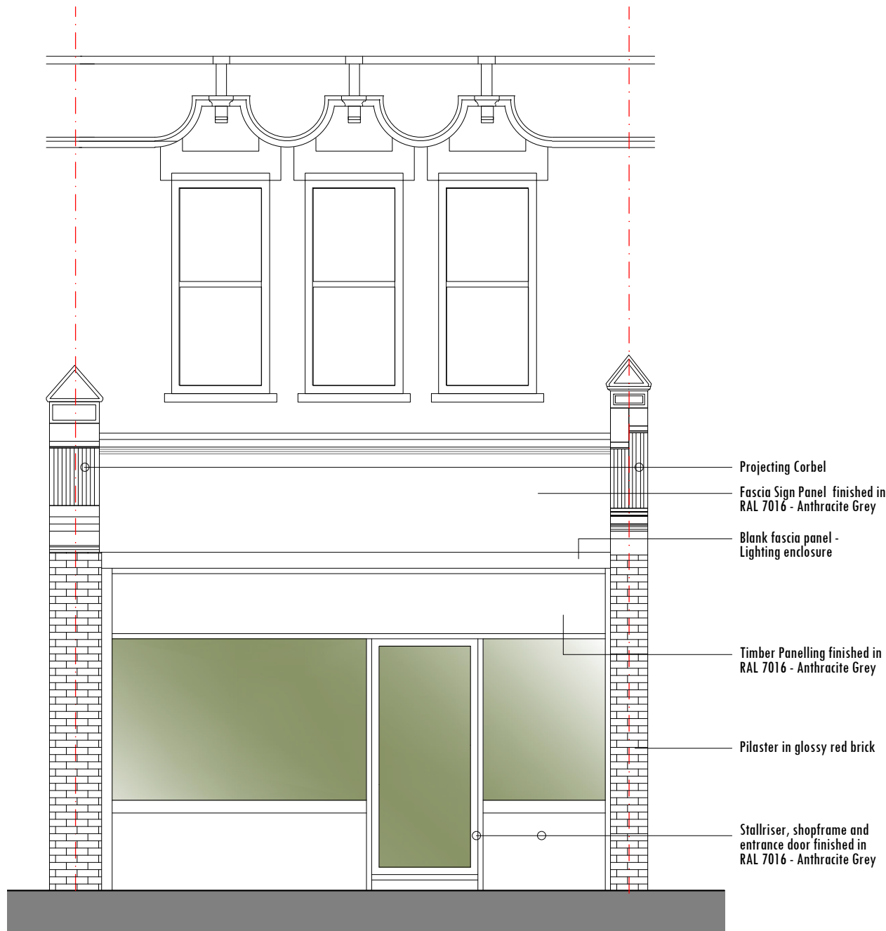
PRE-EXISTING FRONT ELEVATION Scale:1/50
