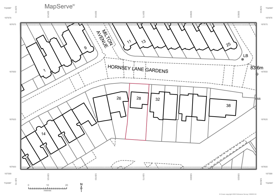
Site Location Plan 1:1250 @A1
