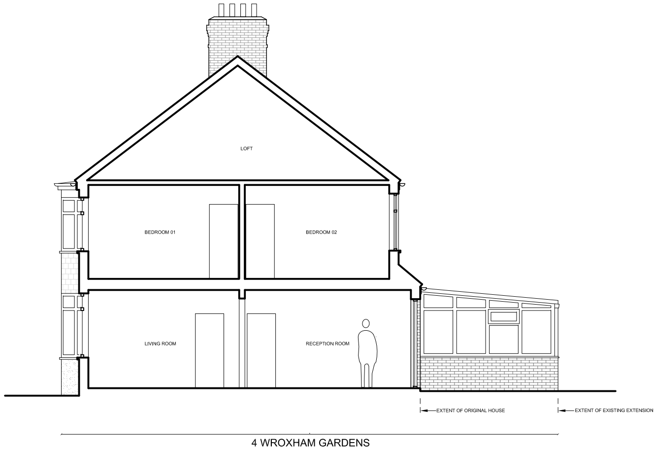
④ CROSS SECTION
