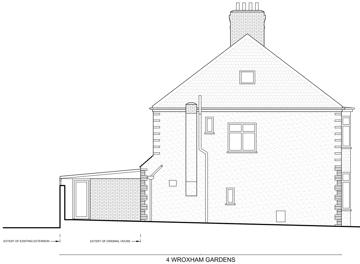
© SIDE ELEVATION
