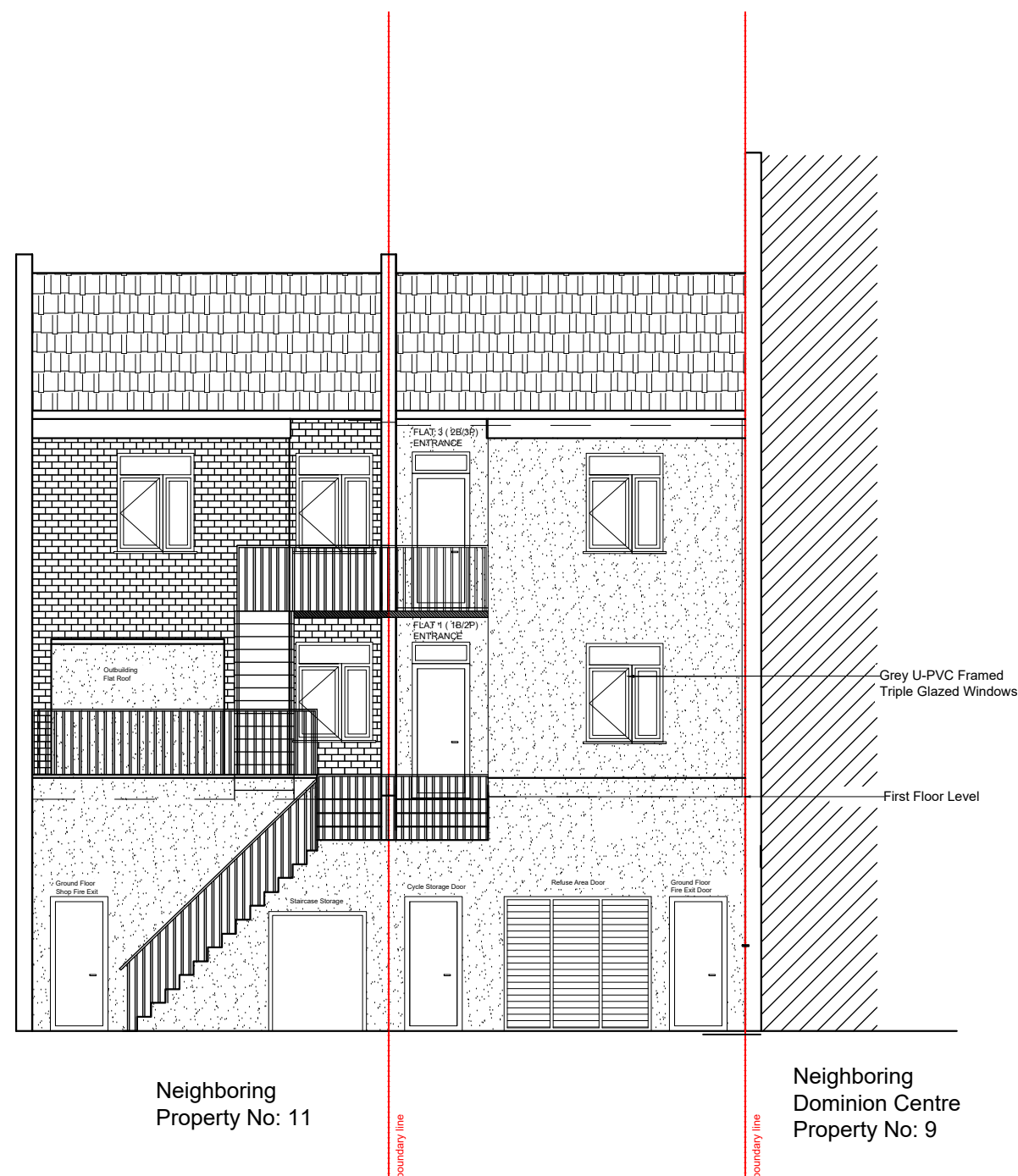
REAR ELEVATION AS PROPOSED
