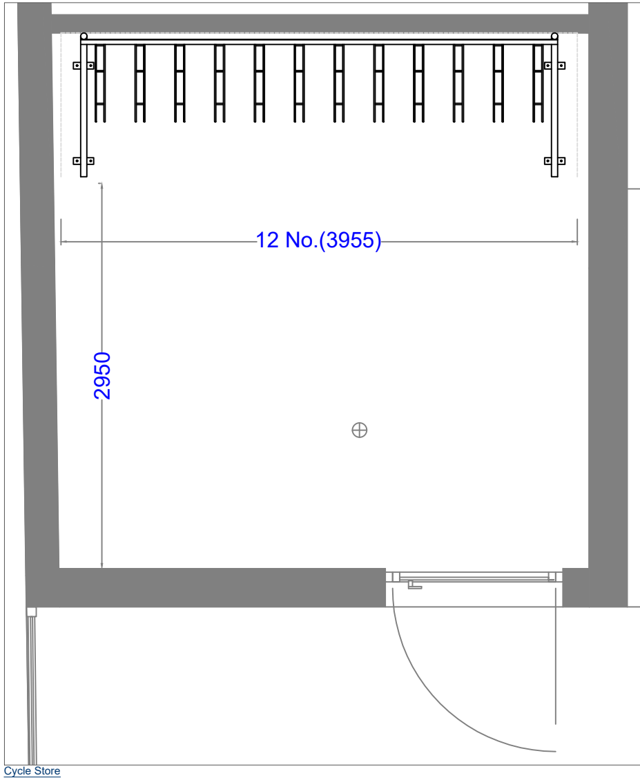
Cycle Store
