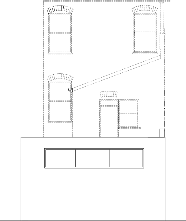
PRE-EXISTING REAR ELEVATION 1:100
