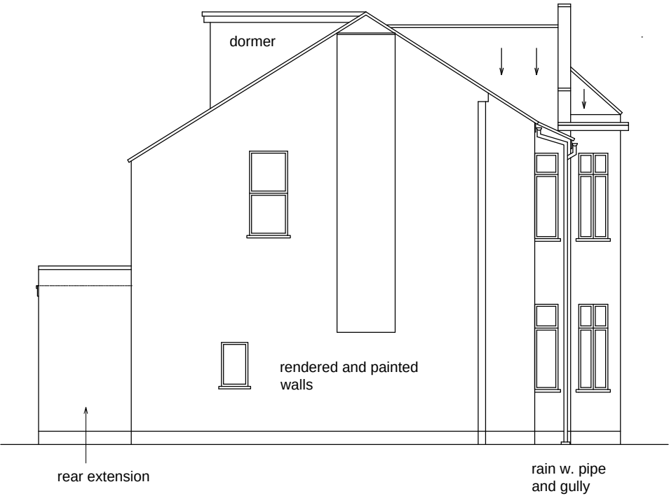
Side elevation (from North) 'As existing' Scale: 1/100
