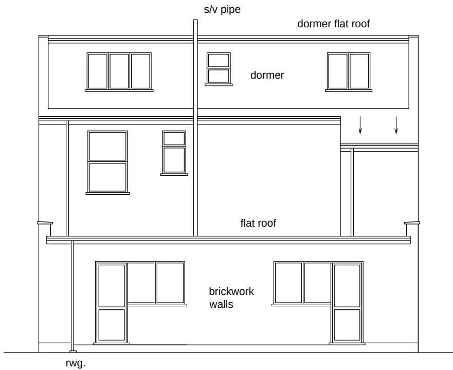
Rear elevation 'As existing' Scale: 1/100
