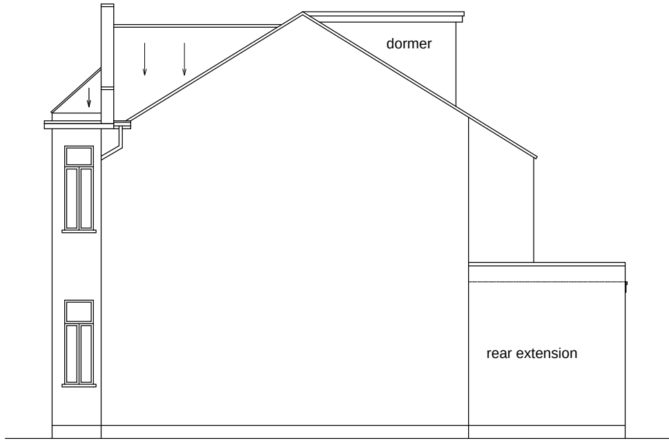
Side elevation (from South) 'As existing' Scale: 1/100
