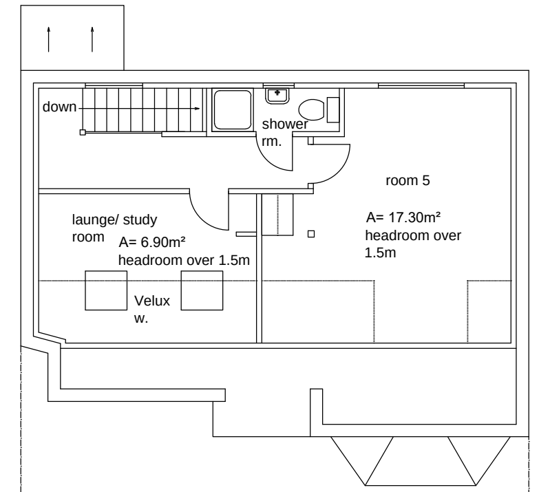
Second floor plan 'As existing' Scale: 1/100
