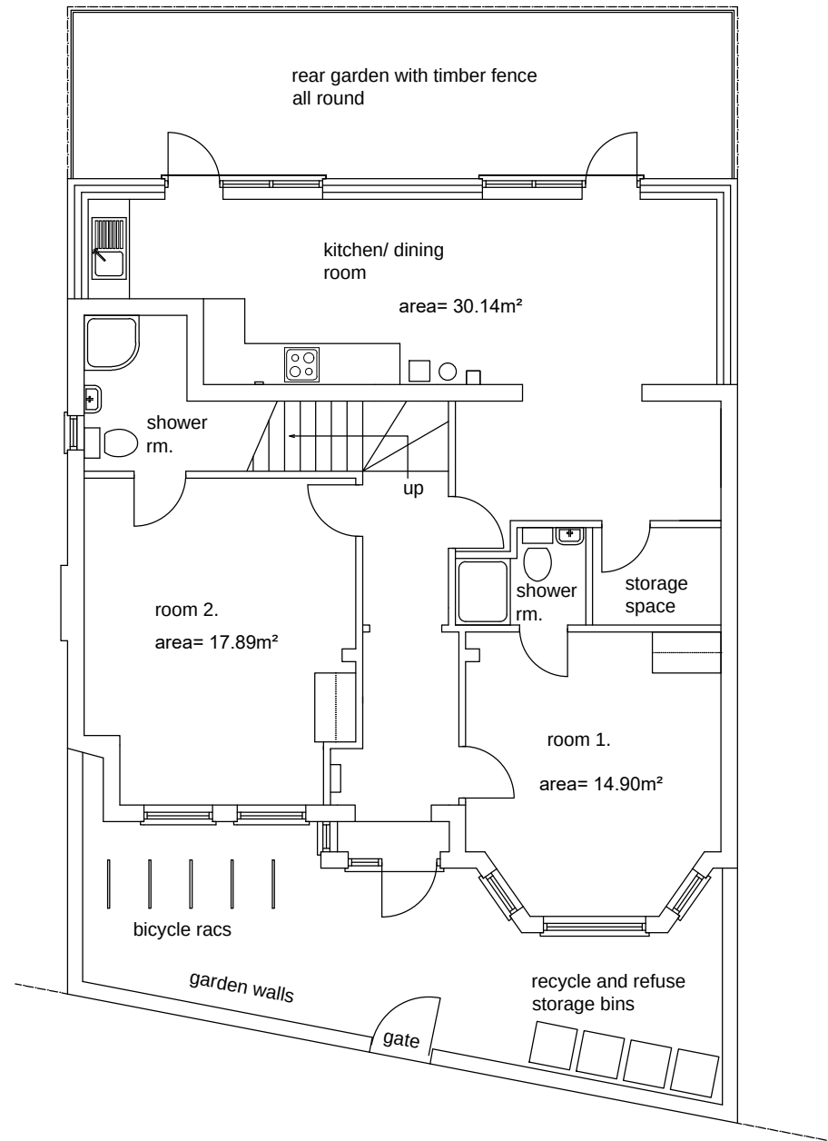
Ground floor plan 'As existing' Scale: 1/100
