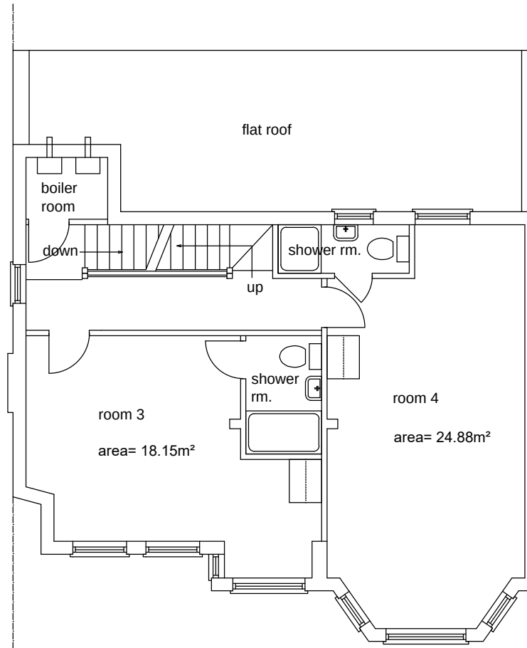
First floor plan 'As existing' Scale: 1/100
