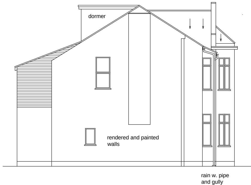
Side elevation (from North) 'As proposed' Scale: 1/100
