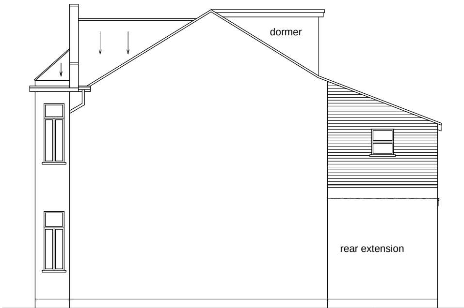
Side elevation (from South) 'As proposed' Scale: 1/100
