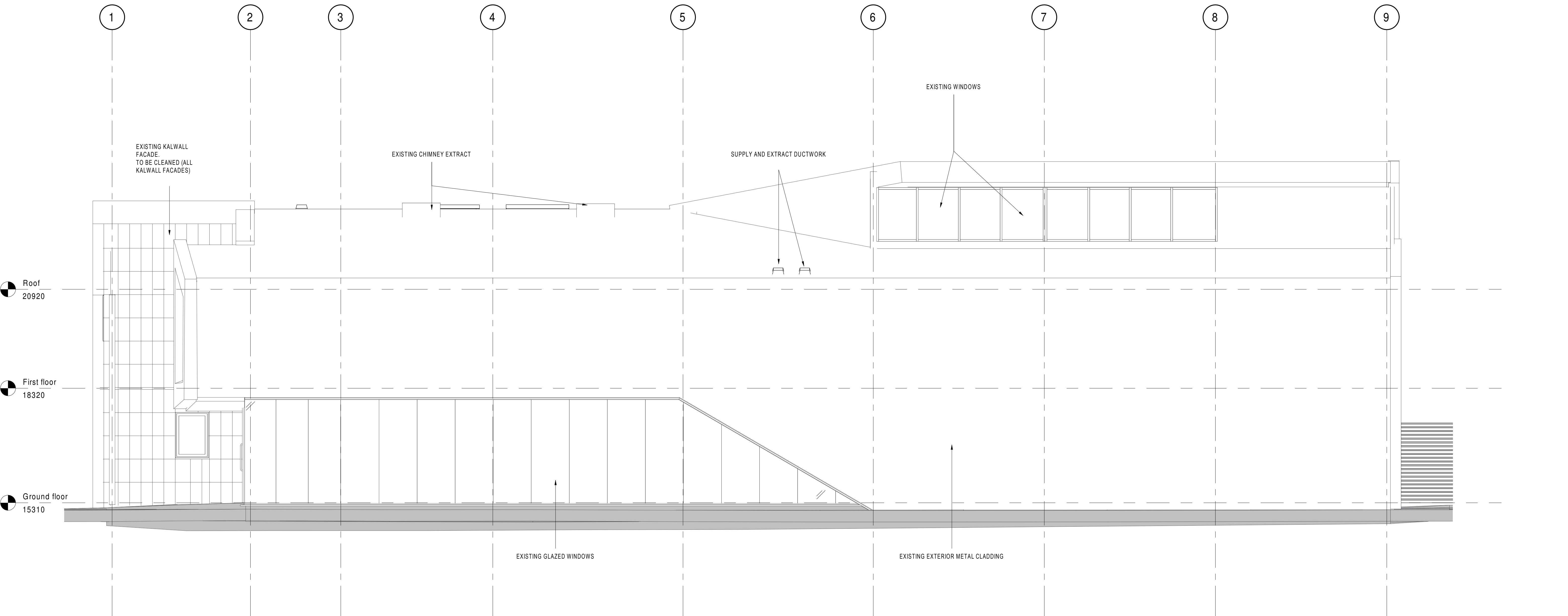
1 PROPOSED SIDE ELEVATION 1 : 50
