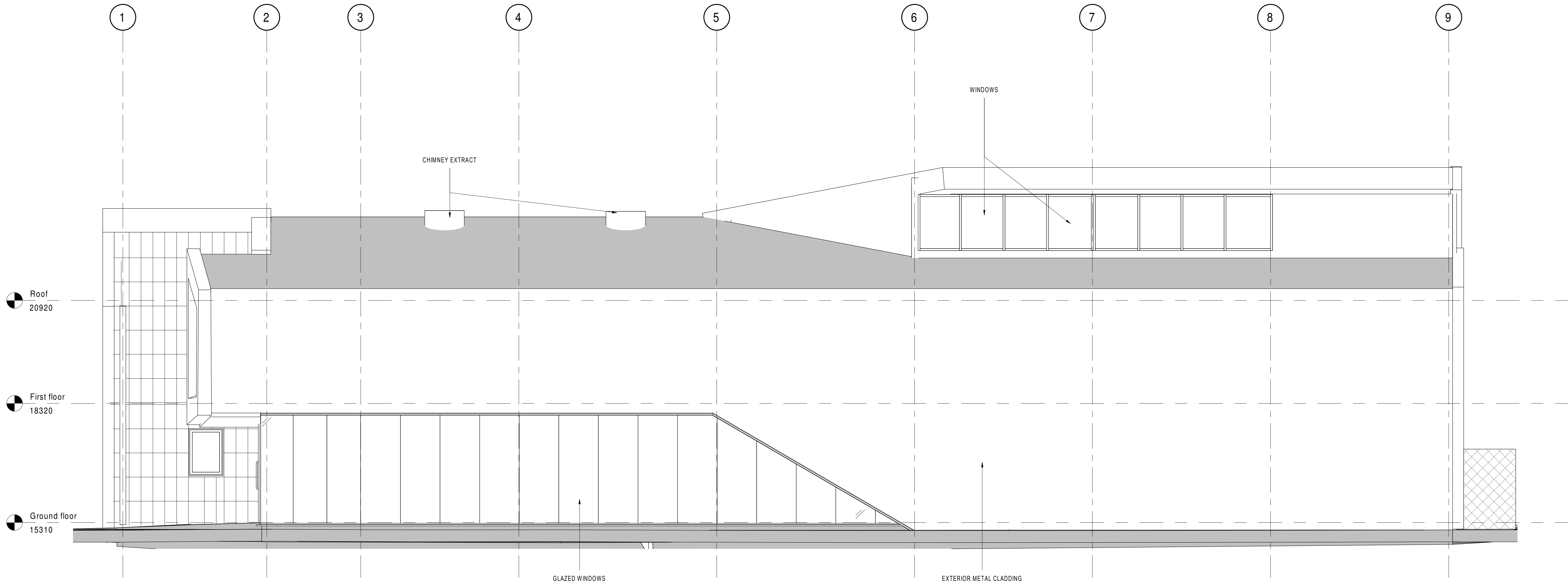
1 EXISTING SIDE ELEVATION 1 1 : 50
