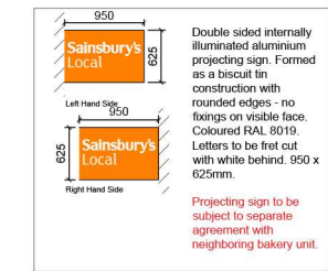
01 PROPOSED FRONT ELEVATION P 94621 210 1:100 @ A3
