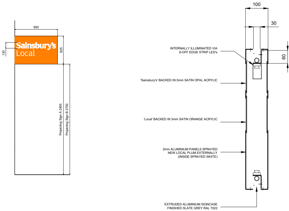
03 PROJECTING SIGN P 94621 213 1:50@A3 ILLUMINATION LEVEL - 204 cd/m 2
