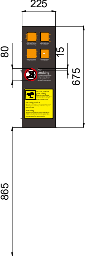
07 STAT SIGN P 94621 213 1:25@A3
