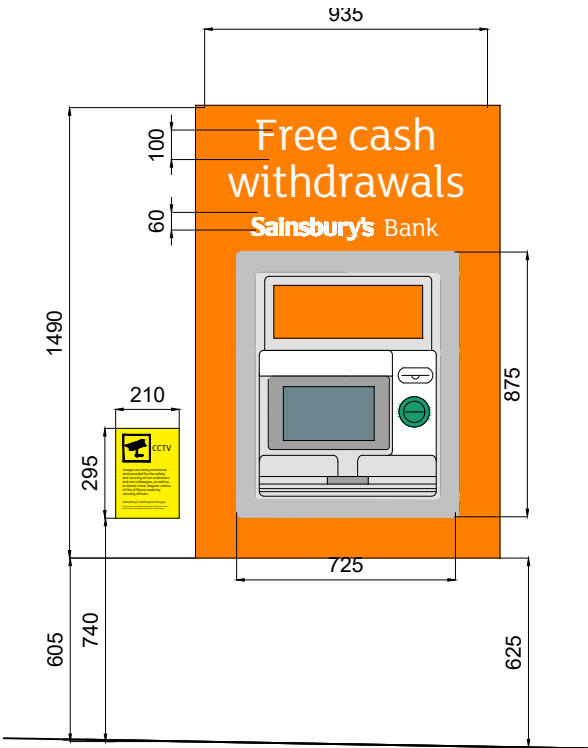
08 ATM SURROUND P 94621 213 1:25@A3
