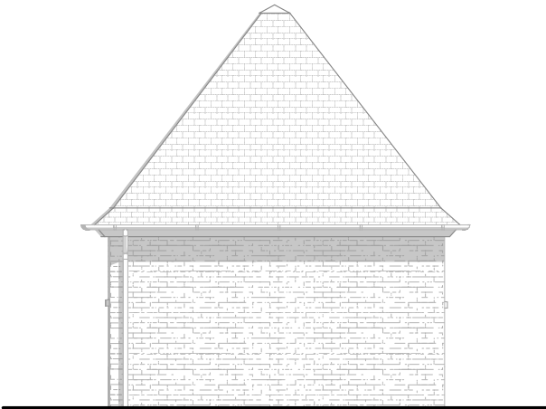
Proposed Side 2 Elevation 1:100
