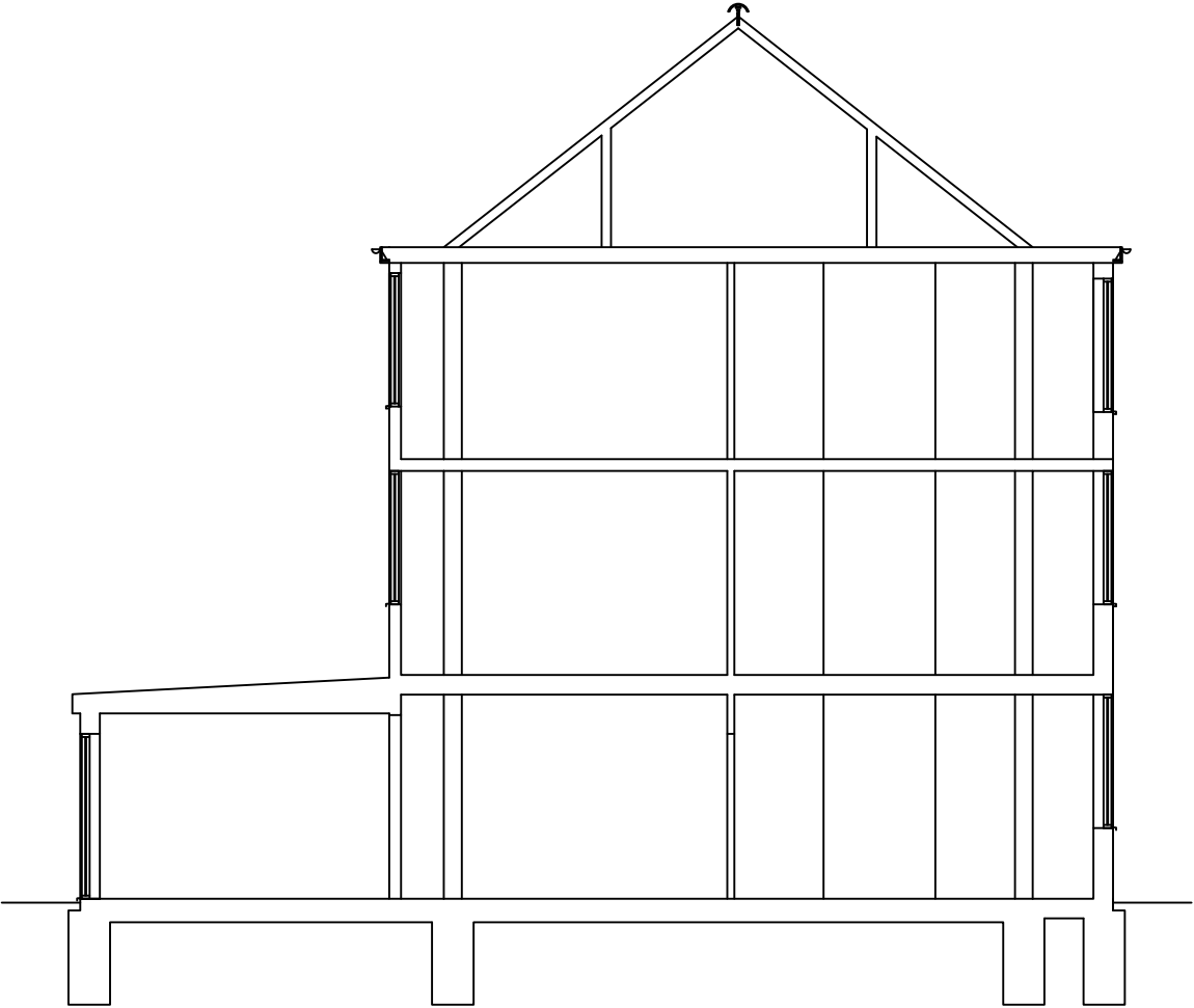
Proposed Section
