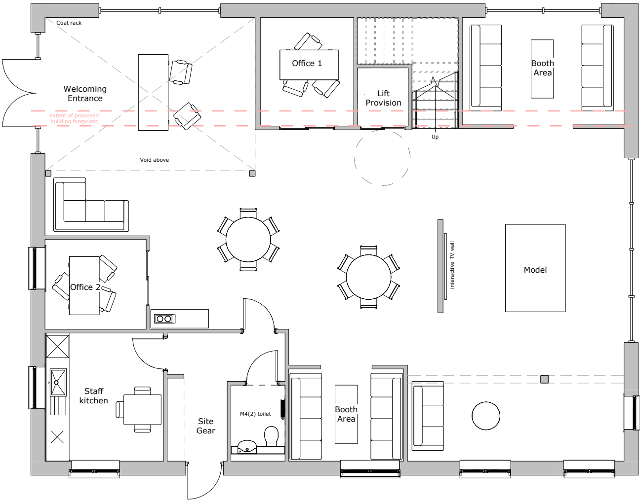
PL-Ground Floor Plan 1 : 100
