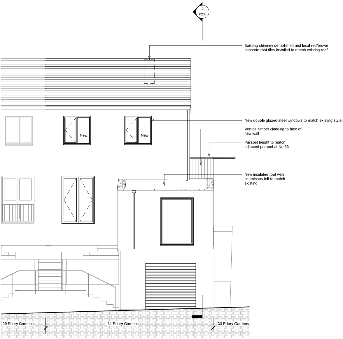
2 Proposed North Elevation 1 : 50
