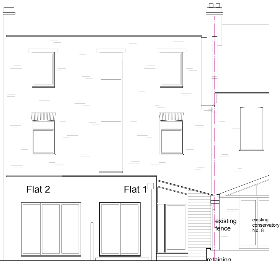
REAR ELEVATION
