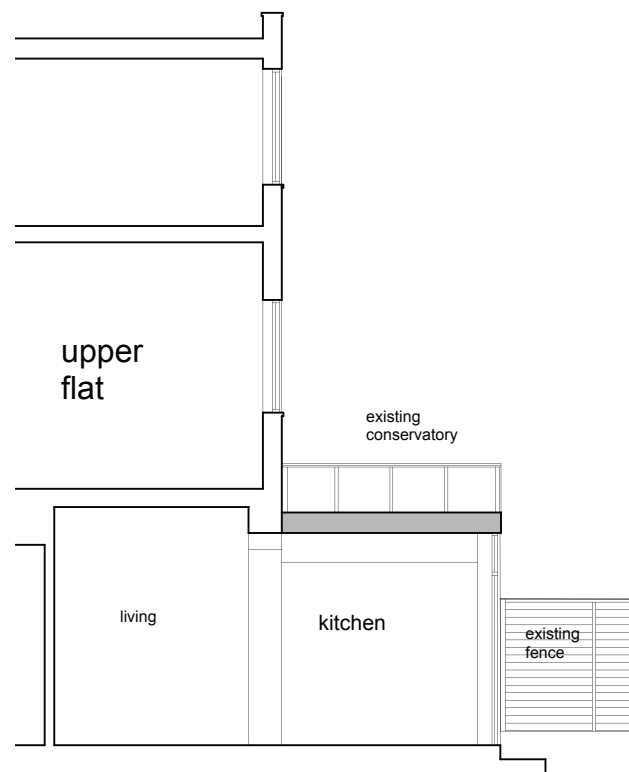
SIDE ELEVATION/SECTION CC - boundary with No. 8
