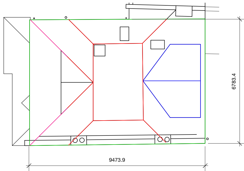
Roof Plan
