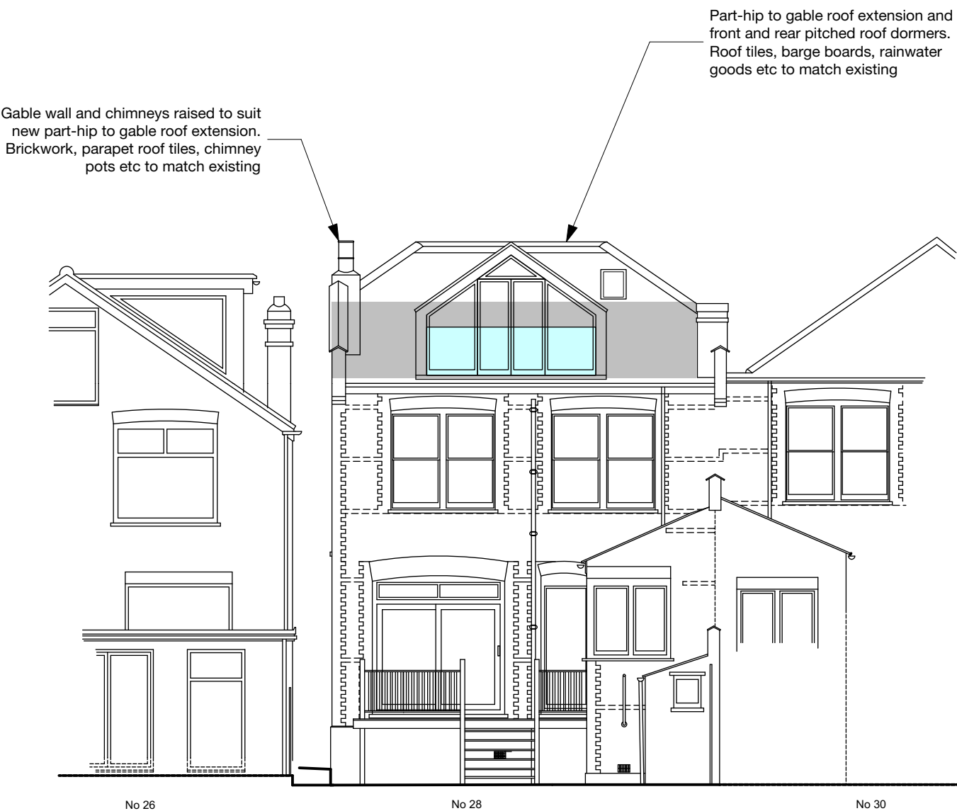
Rear (South-East) Elevation
