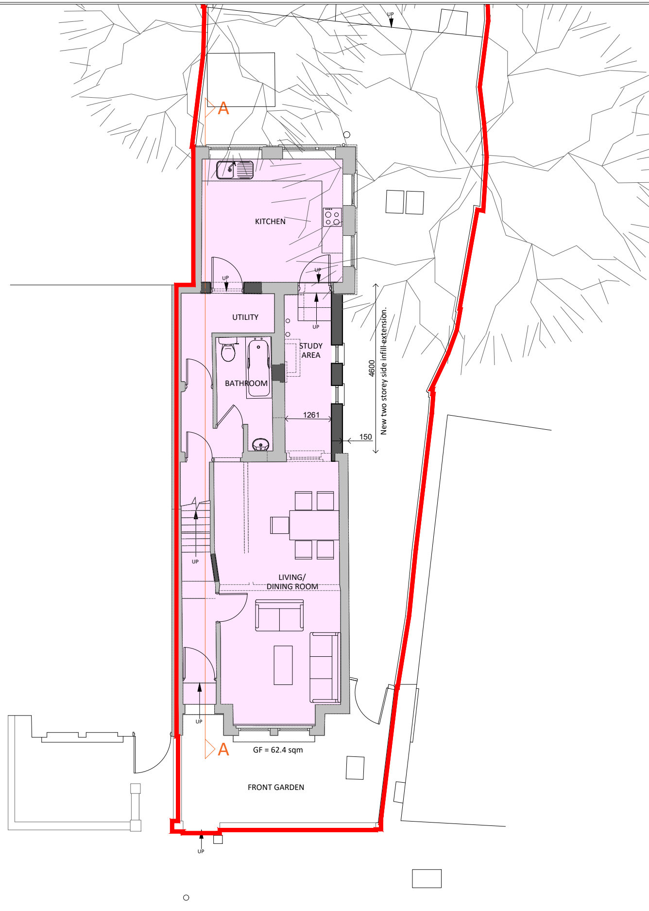
Proposed G Floor Plan
