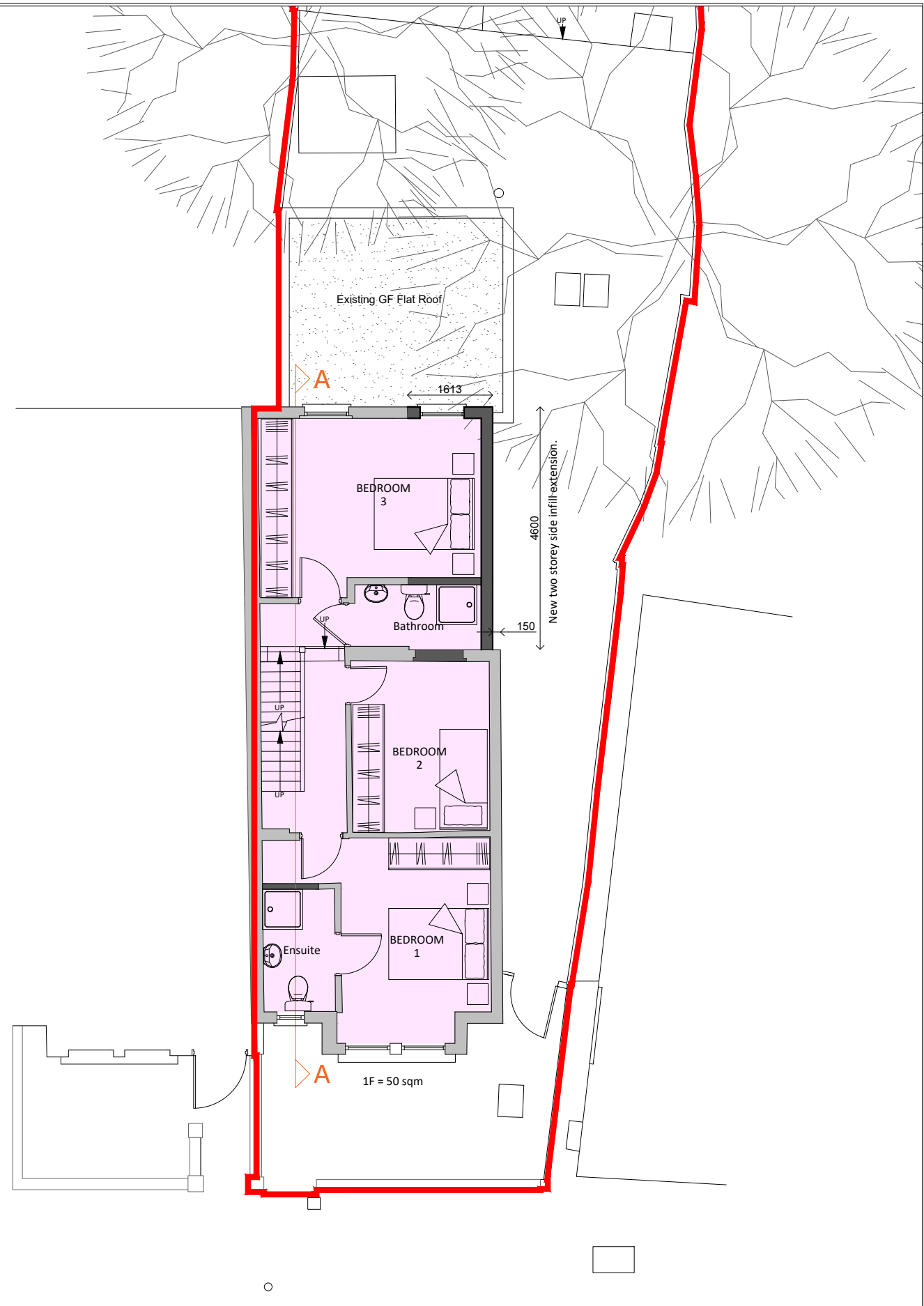
Proposed 1 Floor Plan
