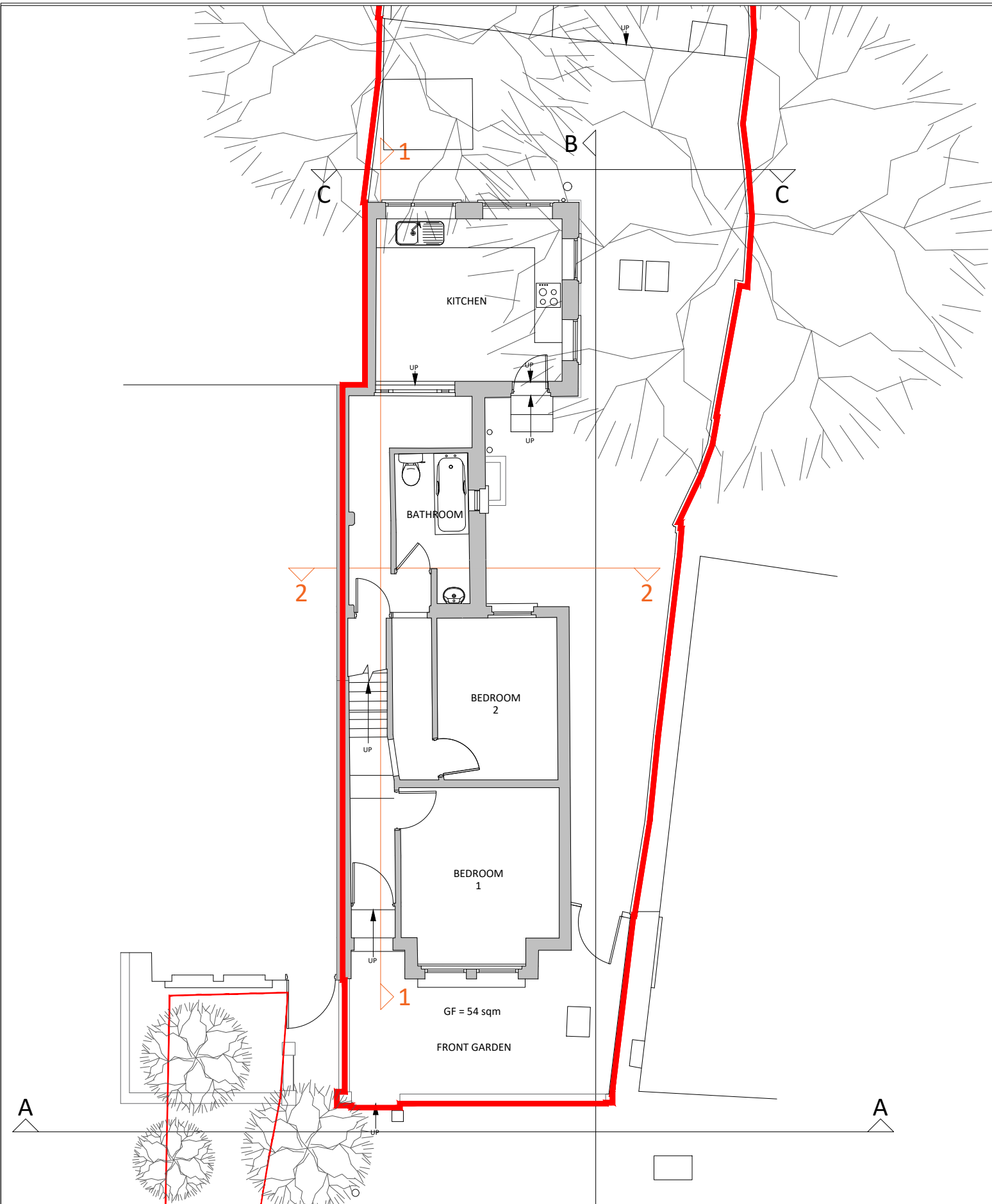
Existing G Floor Plan
