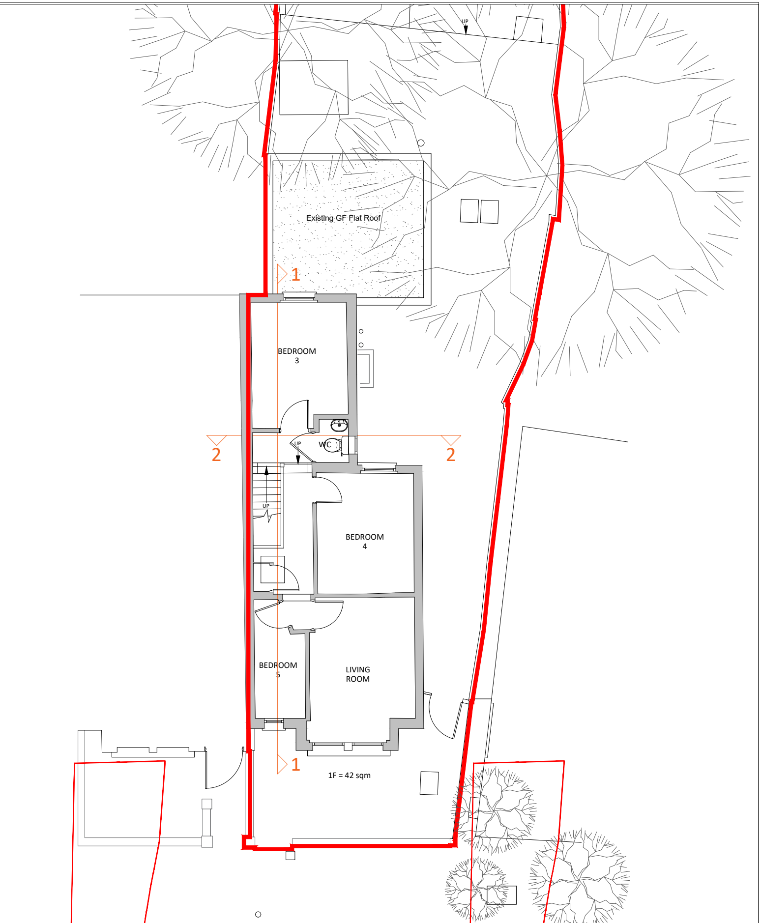
Existing 1 Floor Plan
