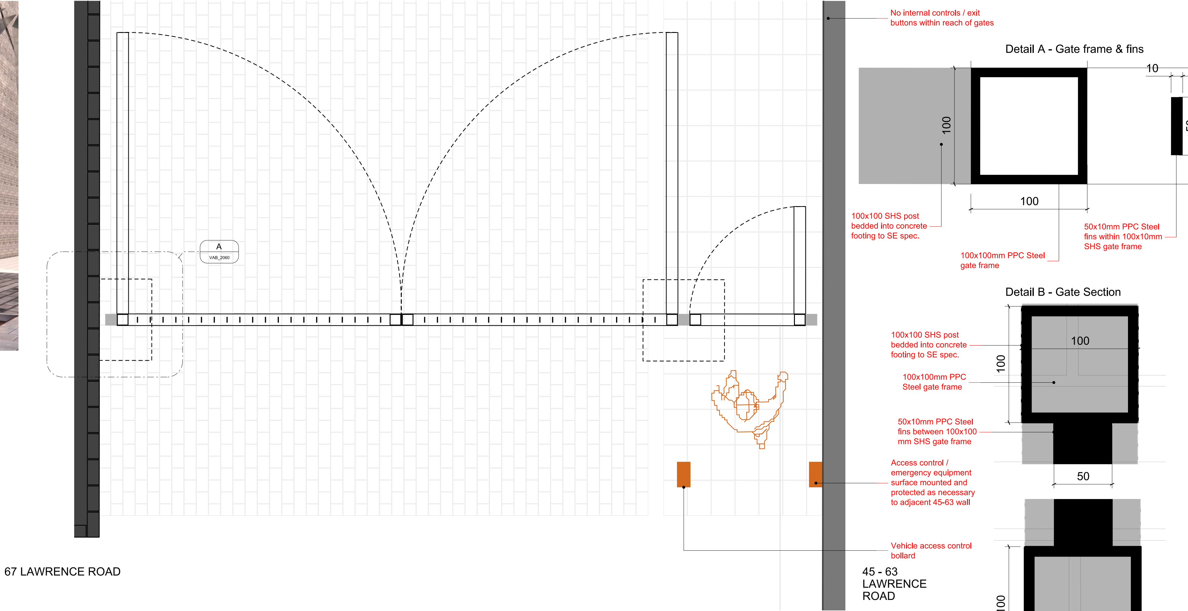
4 Elevation Detail Plan @ 1:20
