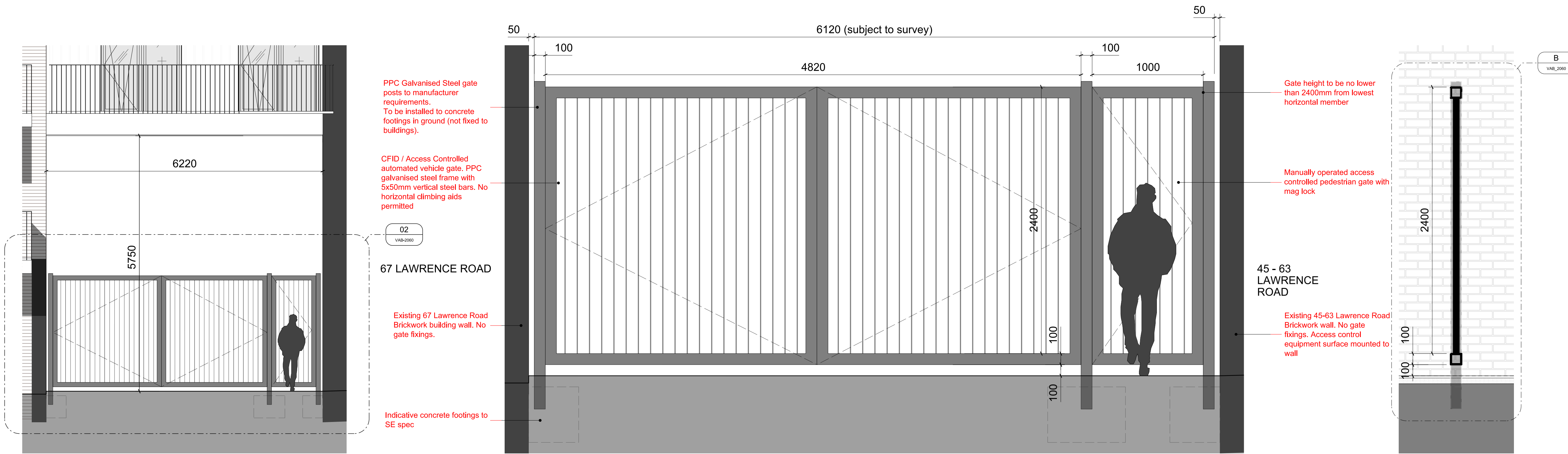
1 Elevation Context Elevation @ 1:50
