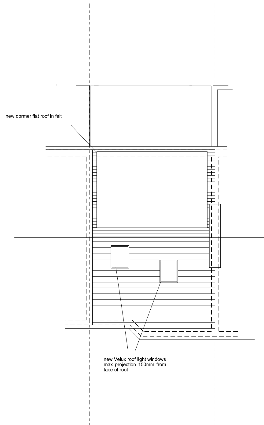
Proposed Roof Floor Plan
