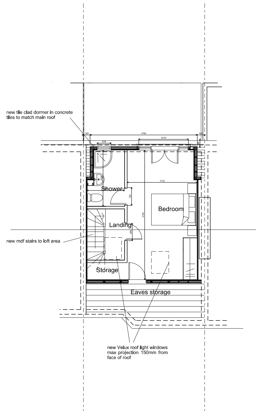
Proposed Second Loft Floor Plan
