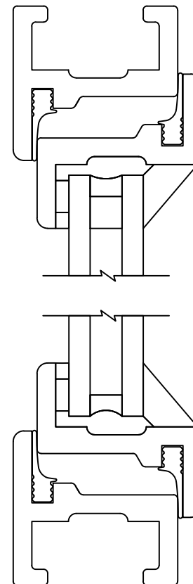
Equal Leg Opening Vertical Section
