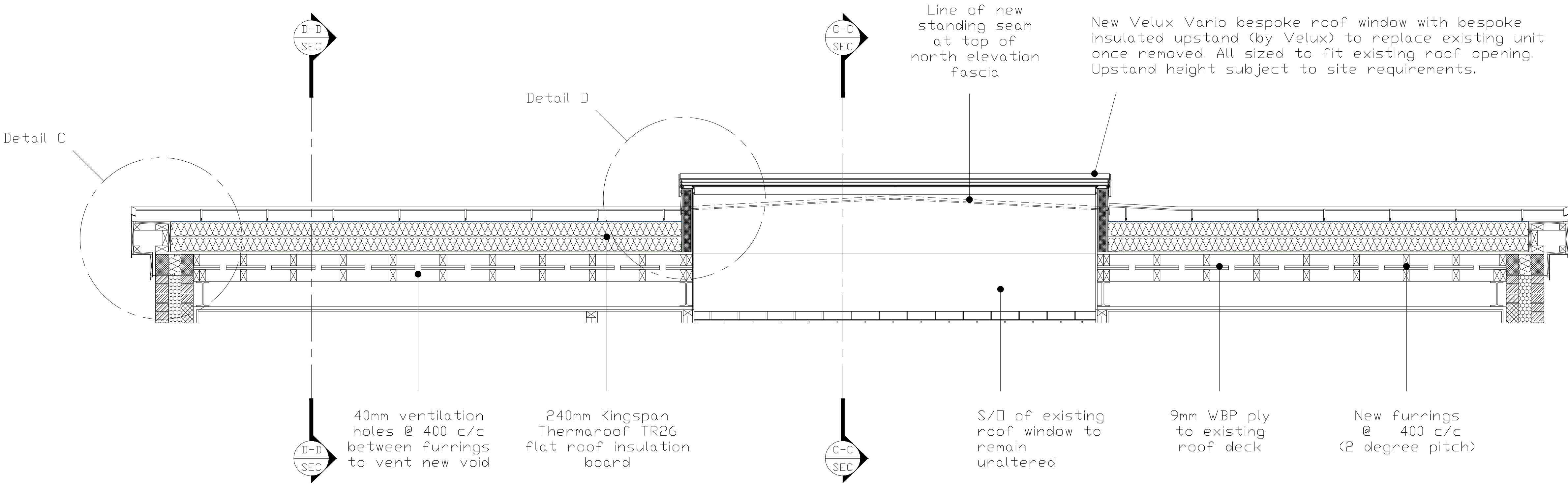
Section B-B
