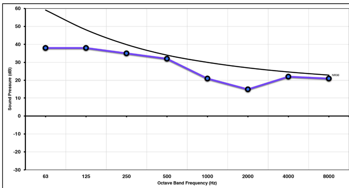
Figure 2 Predicted L_{Amax} noise transfer from AGC to first floor residential bedroom against NR30 noise rating curve
