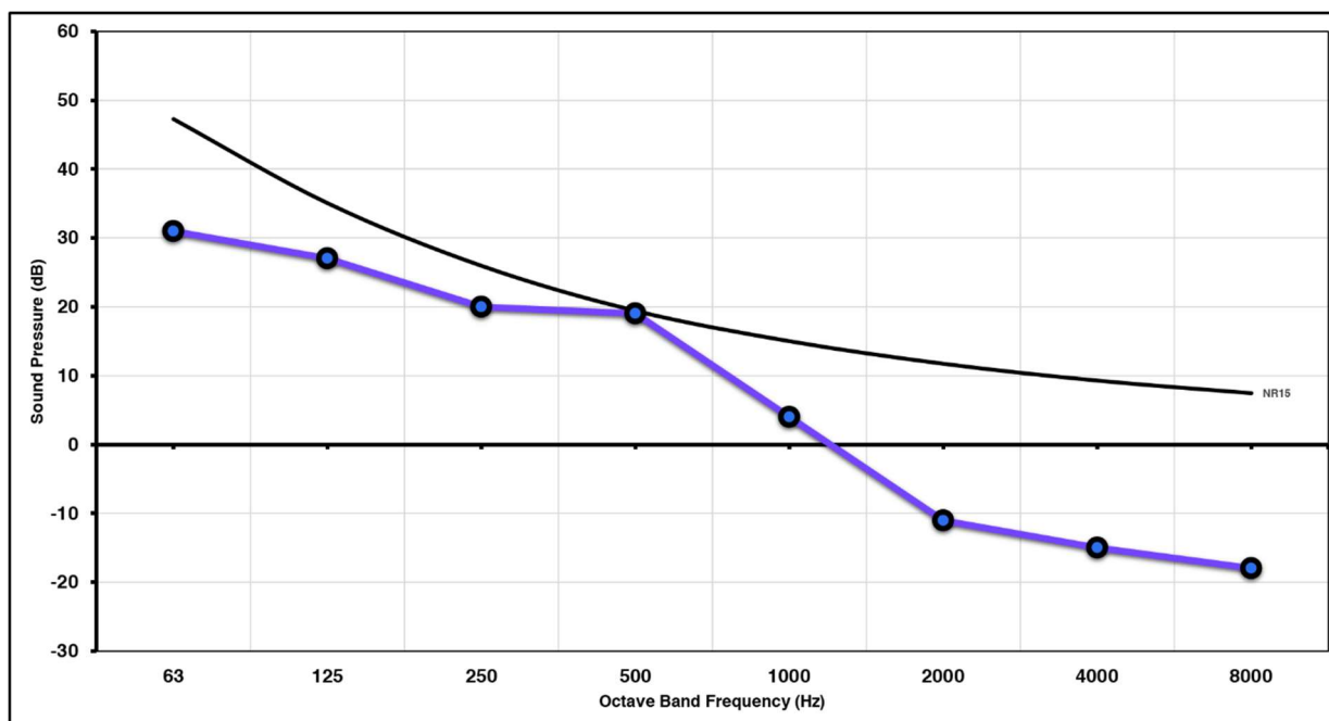
Figure 1 Predicted L_{Aeq} noise transfer from AGC to first floor residential bedroom against NR15 noise rating curve
