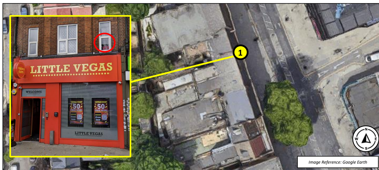
Figure 1 Noise survey measurement location
