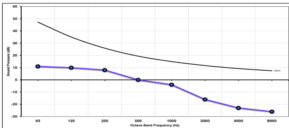
Figure 3 Predicted L_{Aeq} noise breakout from AGC façade to first floor bedroom against NR15 noise rating curve
