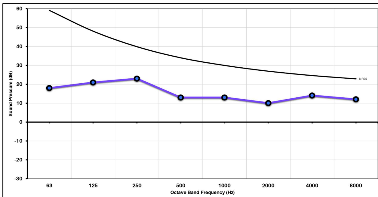
Figure 4 Predicted L_{Amax} noise transfer from AGC to first floor bedroom against NR30 noise rating curve
