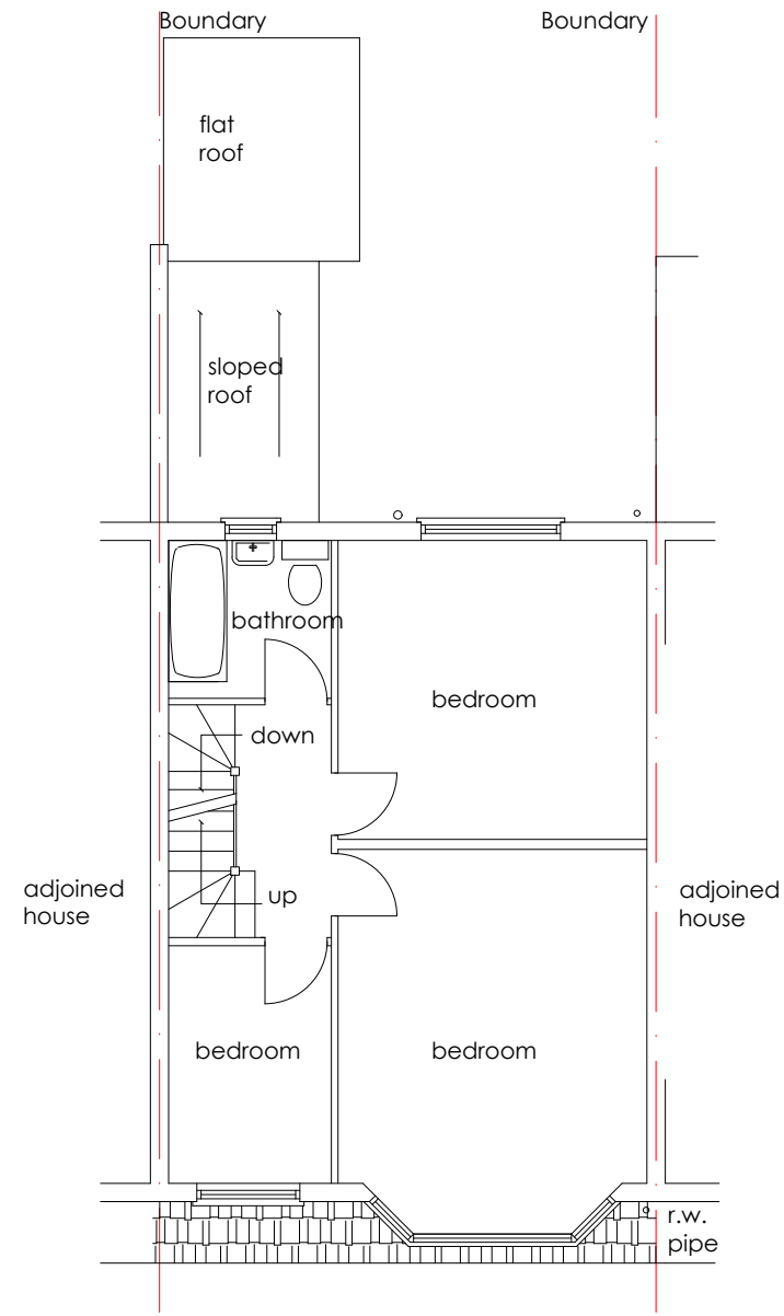
PRE-EXISTING FIRST FLOOR PLAN 1:100
