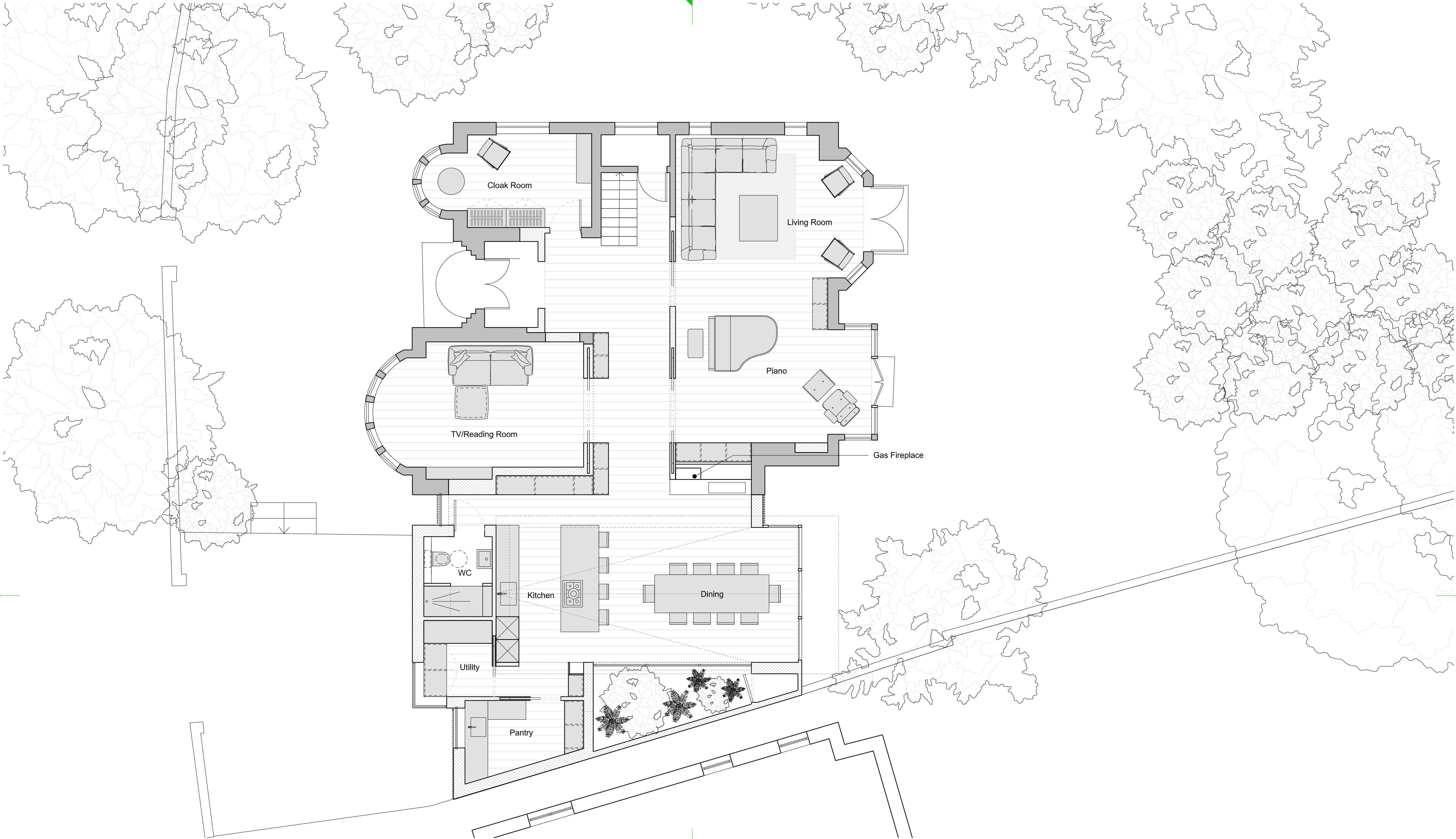
00 Proposed Ground Floor Scale 1:50 @A1 / 1:100 @A3
