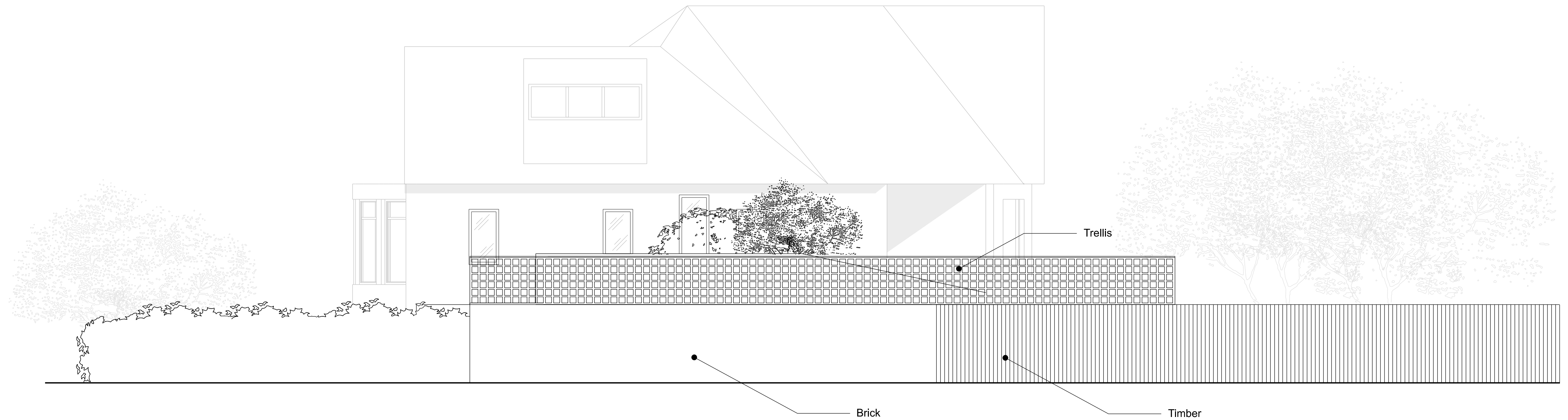
02 Proposed Side Elevation with plants and fence Scale 1:50 @A1 / 1:100 @A3
