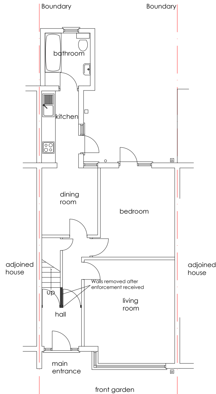
PRE-EXISTING GROUND FLOOR PLAN 1:100
