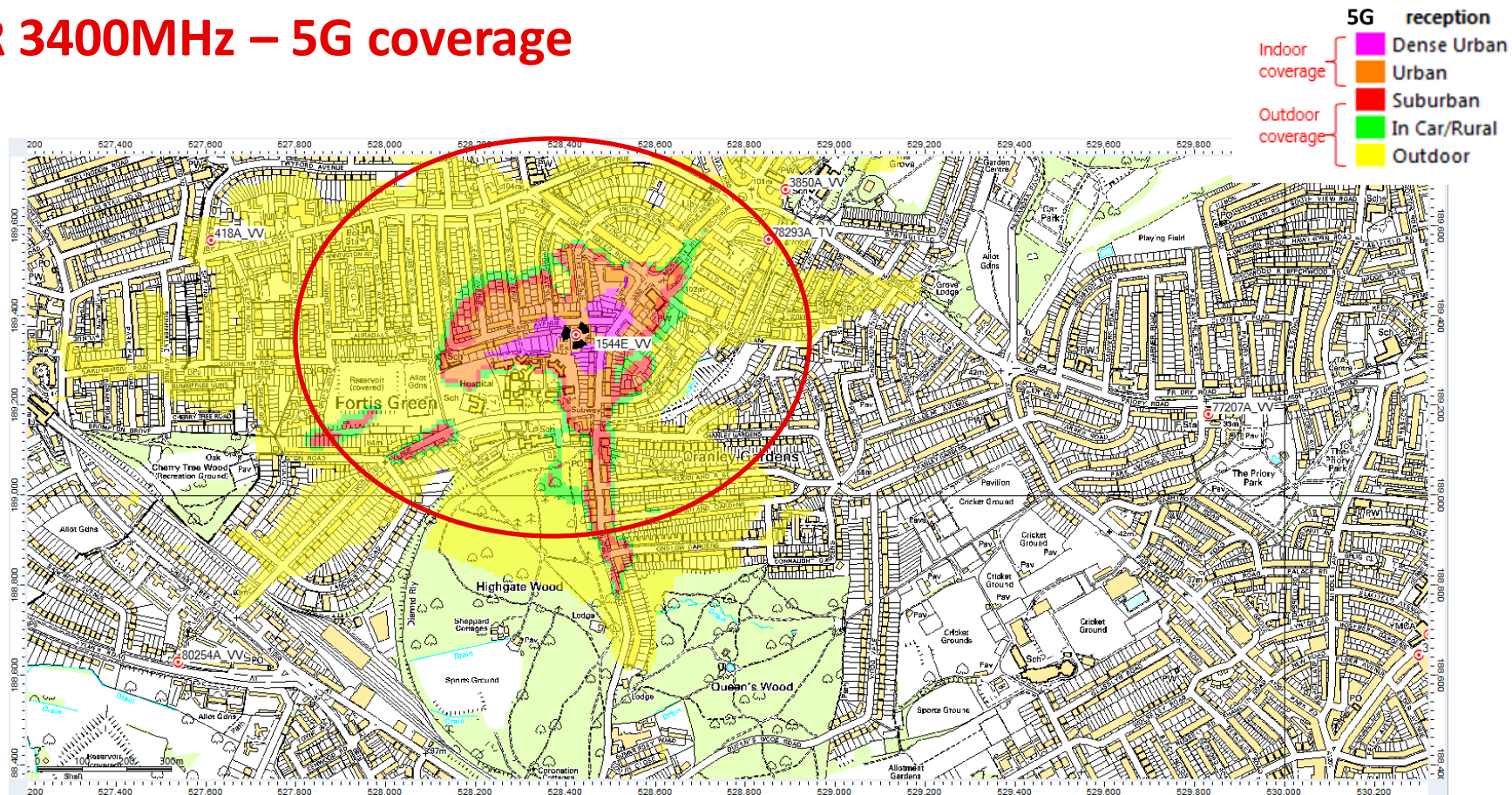
Fig. 2: Proposed NR3400 5G coverage
